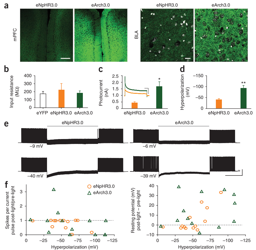
Figure 6 | Performance of hyperpolarizing tools.
