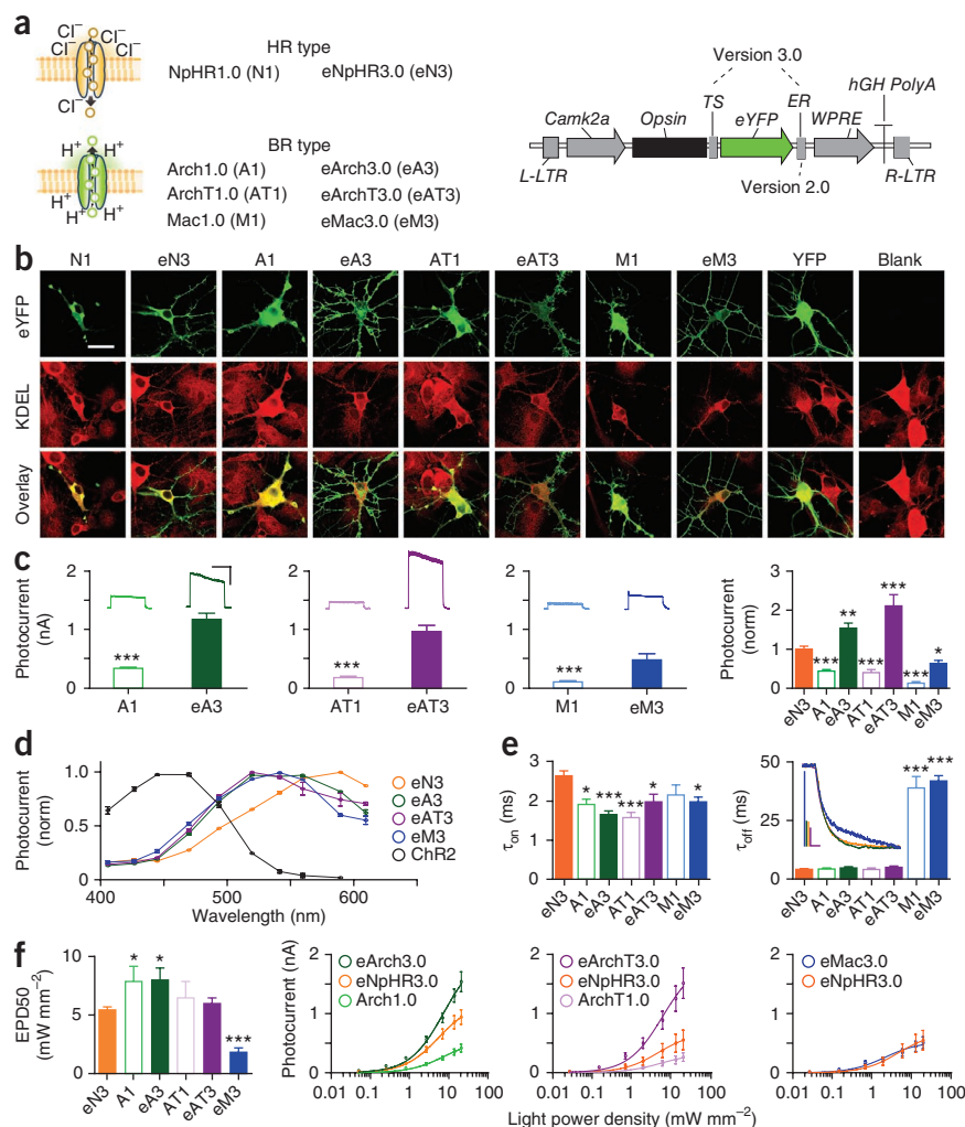
Figure 5 | Properties of hyperpolarizing tools. (a) NpHR is an inward chloride pump (halorhodopsin type; HR), whereas Arch, ArchT, and Mac are outward proton pumps (bacteriorhodopsin type; BR). The 3.0 versions include the endoplasmic reticulum export sequence (ER) after the fluorophore (which constitutes the 2.0 version) as well as a trafficking sequence (TS) between opsin and fluorophore. (b) Confocal images of 1.0 (the originally described version of the molecule) and 3.0 versions (green) expressed in culture and immunolabeled with an ER marker (KDEL; red). Scale bar, 25 \mu\text{m} . (c) Representative traces and raw photocurrents in response to 1 s light for 1.0 (open bars) versus 3.0 versions (closed bars) for Arch ( n = 15 –19), ArchT ( n = 14 –16) and Mac ( n = 8 –12). Vertical and horizontal scale bars represent 500 pA and 500 ms, respectively. Photocurrents were normalized to eNpHR3.0 values from within the same experiment to enable direct comparisons across opsins ( n = 8 –35). (d) Action spectra for 3.0 versions ( n = 7 –20) alongside ChR2 (black). (e) \tau_{\text{on}} and \tau_{\text{off}} ( n = 7 –35). Vertical and horizontal scale bars represent 200 pA and 5 ms, respectively. (f) EPD50 values for all hyperpolarizing opsins ( n = 5 –14). Raw photocurrent versus light power density plotted alongside within-experiment eNpHR3.0 ( n = 5 –14). Population data are plotted as mean \pm s.e.m. * P < 0.05 , ** P < 0.01 and *** P < 0.001 . Unless otherwise indicated, eNpHR3.0 was activated with 590-nm light, and all other tools were activated with 560-nm light, both at \sim 5 \text{ mW mm}^{-2} .
